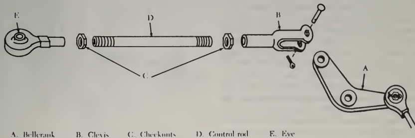
FIGURE 8-8. Engine control linkage assembly.
